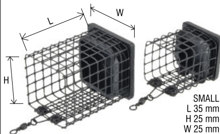
BIG L 55 mm H 40 mm W 40 mm
